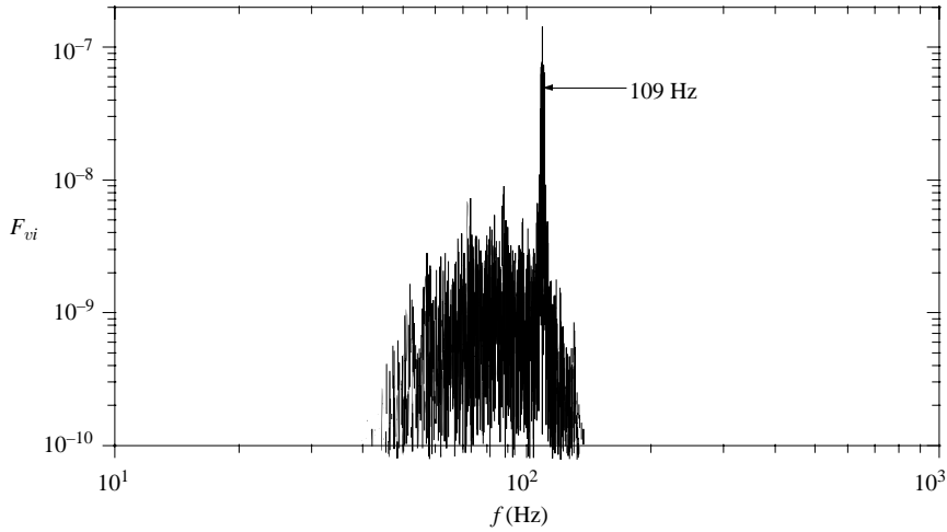
FIGURE 3. Spectra of the wavelet component at f_0 (wavelet level 9) of the v -signal at y/d \approx 0.7 .
